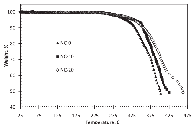
Figure 4 TGA thermograms of NC-0 and composite sample NC-10 and NC-20.
